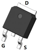
TO-252-4R(DPAK) top view
